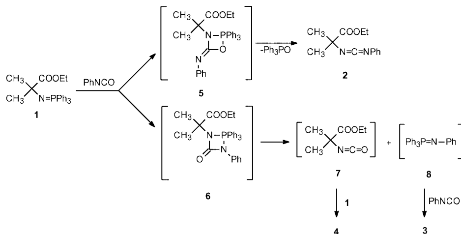
Scheme 2. Proposed mechanism of the abnormal aza-Wittig reaction leading to two different carbodiimides versus that of the normal aza-Wittig reaction.
