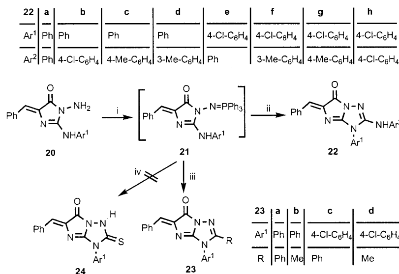
Scheme 7. (i) Ph 3 P, C 2 Cl 6 , CH 2 Cl 2 , NEt 3 , room temp.; (ii) Ar 2 NCO, 1–2 h; (iii) RCOCl, 2–3 h. (iv) CS 2 , 2 h.
