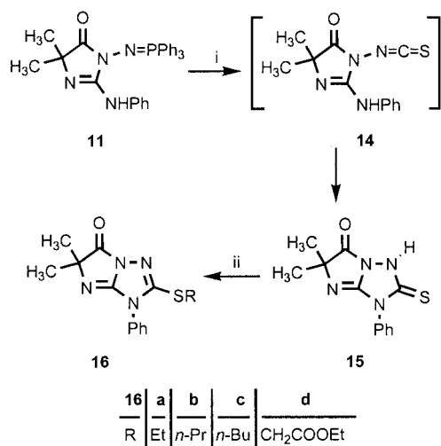
Scheme 5. Reaction conditions: (i) CS 2 , CH 2 Cl 2 , 40 °C, 3 h; (ii) RX, CH 3 CN, K 2 CO 3 (s), room temp. or 50–60 °C, 1–4 h.
