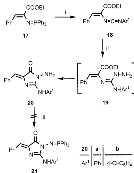
Scheme 6. Reaction conditions: (i) Ar 1 NCO, CH 2 Cl 2 , room temp., 4–6 h; (ii) NH 2 NH 2 , EtOH, room temp., 10 min; (iii) Ph 3 P, C 2 Cl 6 , CH 3 CN, NEt 3 , room temp., 4–6 h.
