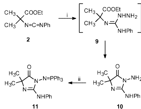
Scheme 3. Reaction conditions: (i) \text{NH}_2\text{NH}_2 , \text{CH}_3\text{CN} , room temp., 2 h; (ii) \text{Ph}_3\text{P} , \text{C}_2\text{Cl}_6 , \text{CH}_3\text{CN} , \text{NEt}_3 , room temp., 4–6 h.
