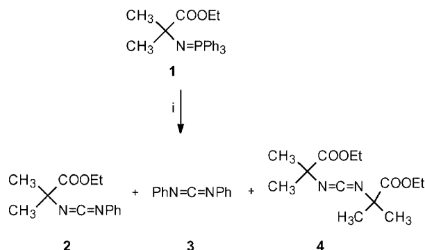
Scheme 1. Reaction conditions: (i) PhNCO, CH 2 Cl 2 , room temp., 2 h.
