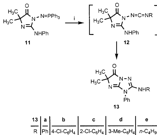
Scheme 4. Reaction conditions: (i) \text{Ar}^1\text{NCO} , \text{CH}_2\text{Cl}_2 , room temp., 1–2 h.
